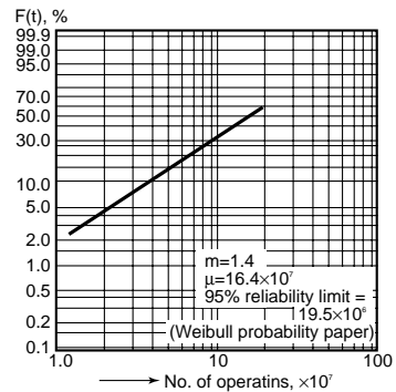
14.-(2) Contact reliability (100 mA 5 V DC resistive load) Tested sample: TQ2-12V Condition: Detection level 100 W
