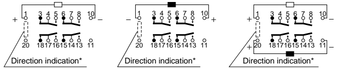
Schematic (Bottom view)
