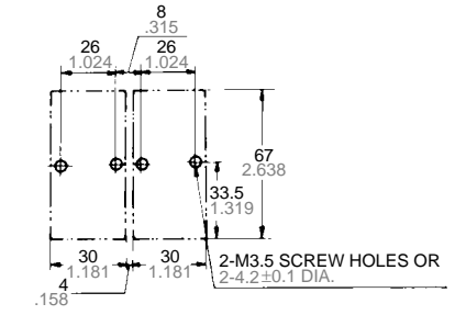
Layout for tandem mounting
