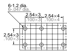
PC board pattern (Copper-side view) Single side stable
